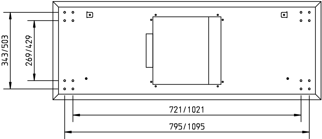
Plan View Showing Fixing Holes Centres
