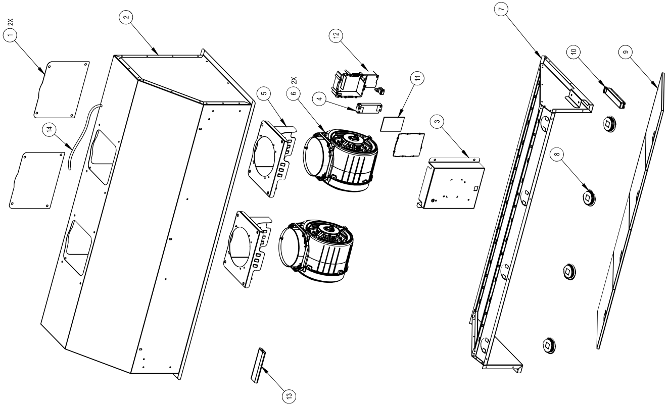
BLOQUE PRO 1200 / 1500 EXPLODED VIEW INTERNAL MOTOR
