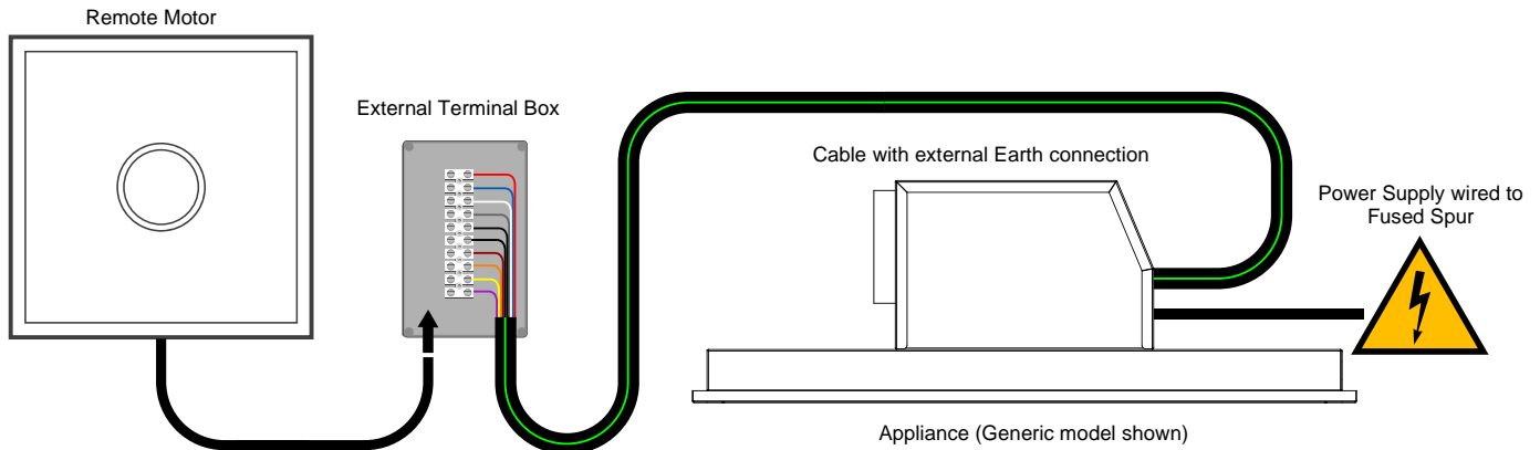
Fig. 1 Typical System
