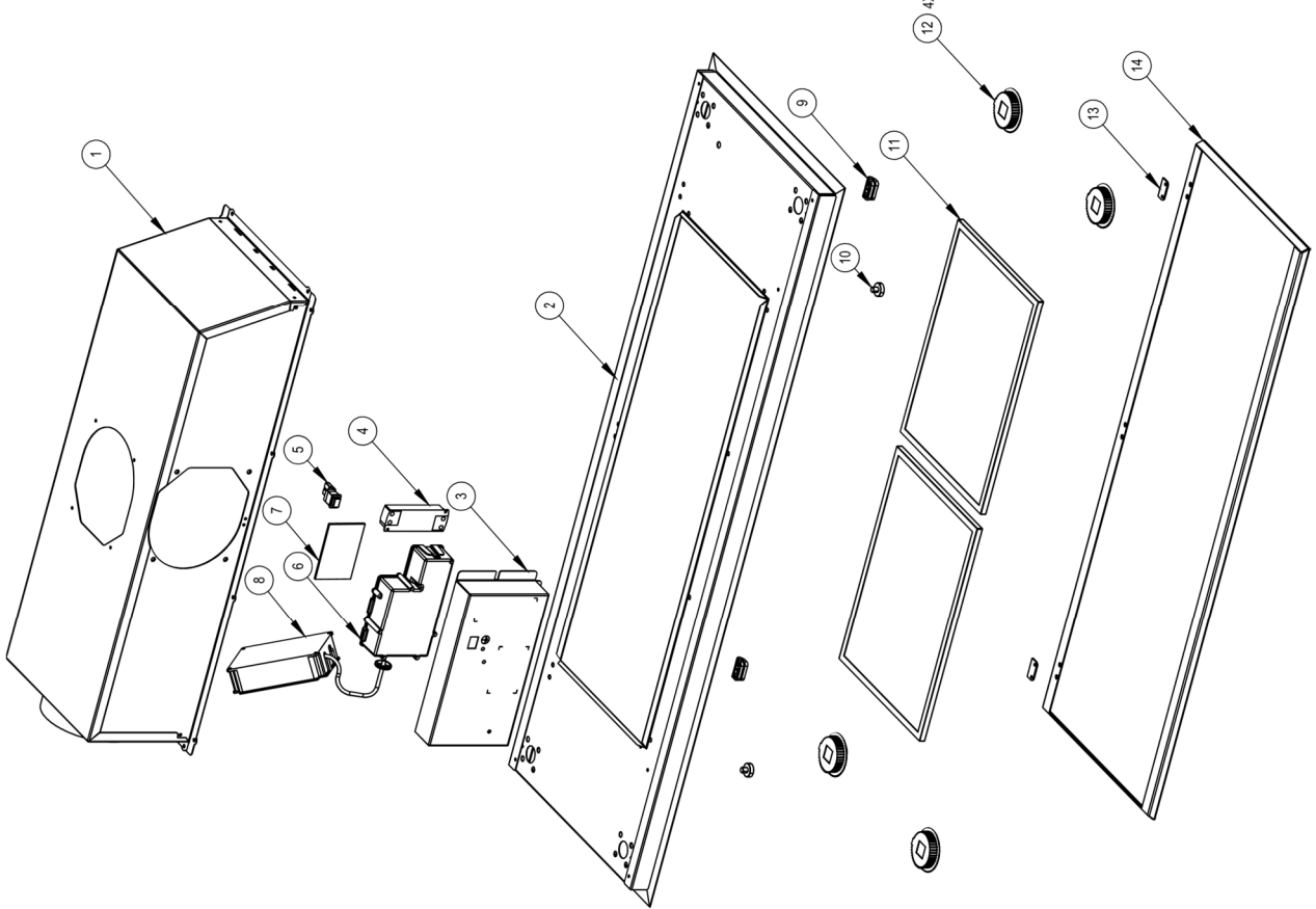
WSW Stratus External Motor – Exploded View
