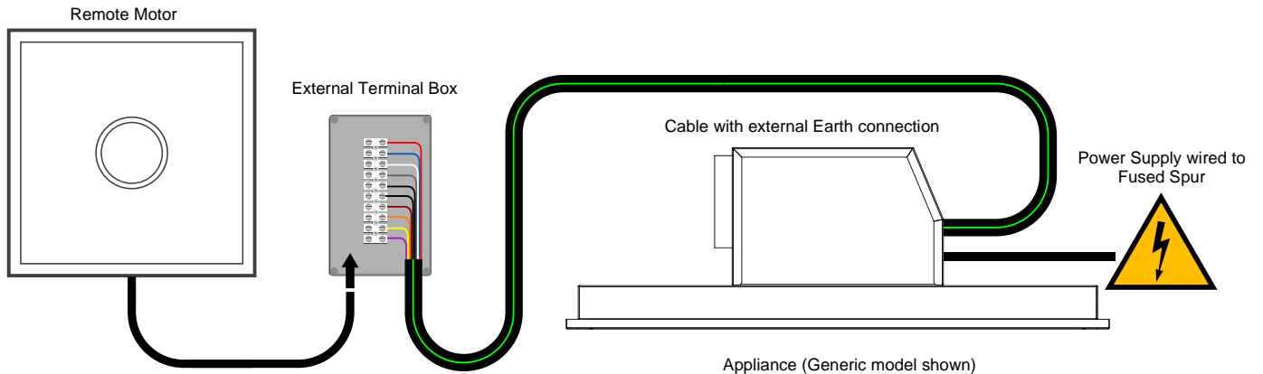
Fig. 1 Typical System
