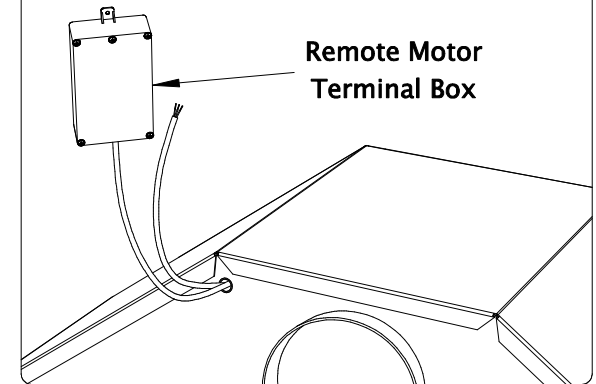
Remote Motor Version With remote motor terminal box exiting alongside electrical supply lead
